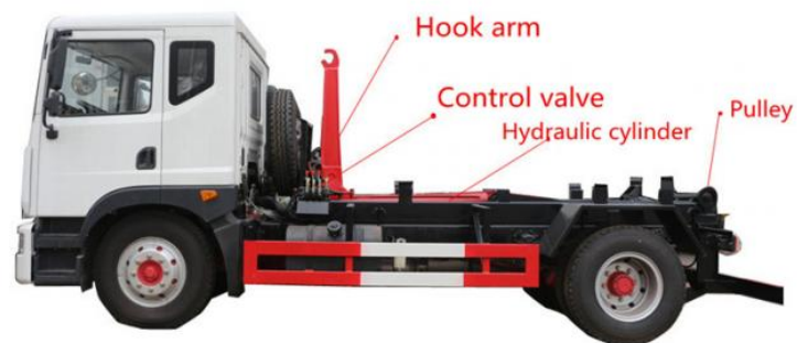
Hook Arm Lifting Garbage Truck Details
